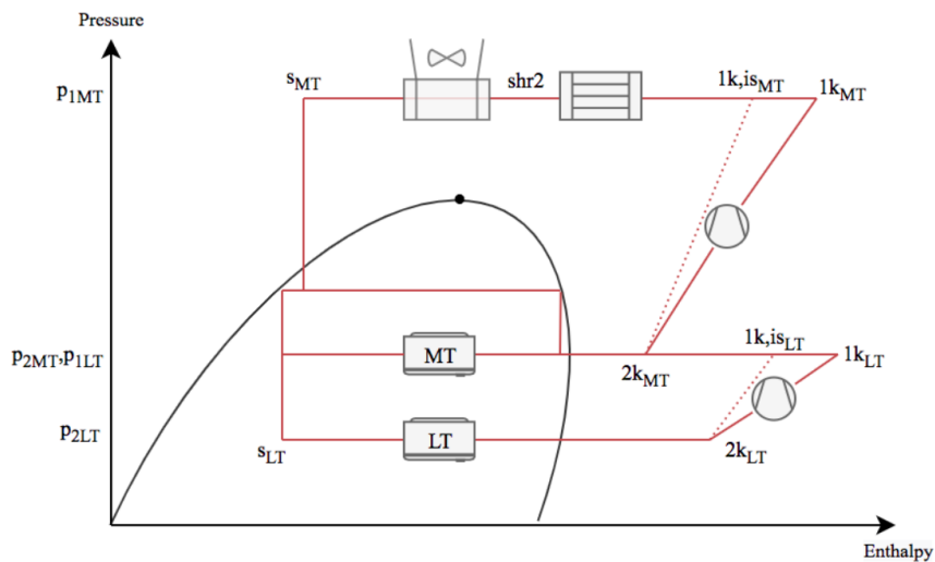
Figure 2: The CO 2 booster refrigeration system in an enthalpy-pressure diagram (Almebäck & Magnus, 2022)
